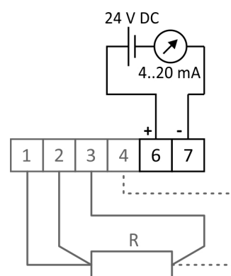
Figure 14.8: Transmitter wiring diagram
