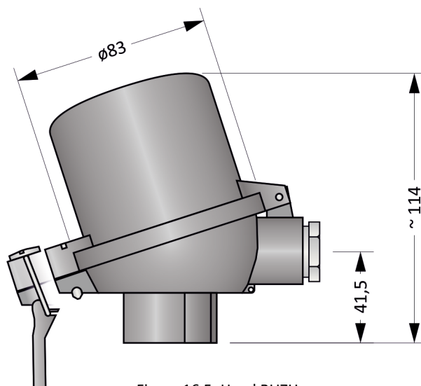
Figure 16.5: Head BUZH
