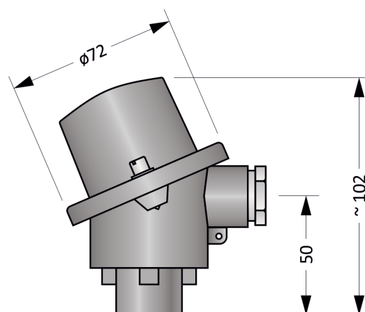
Figure 16.3: Head BH
