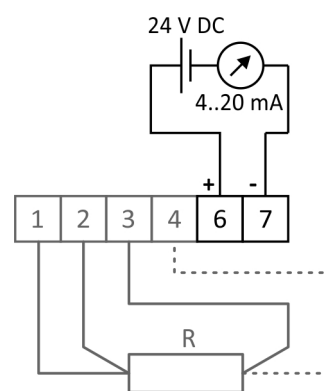
Figure 16.8: Transmitter wiring diagram
