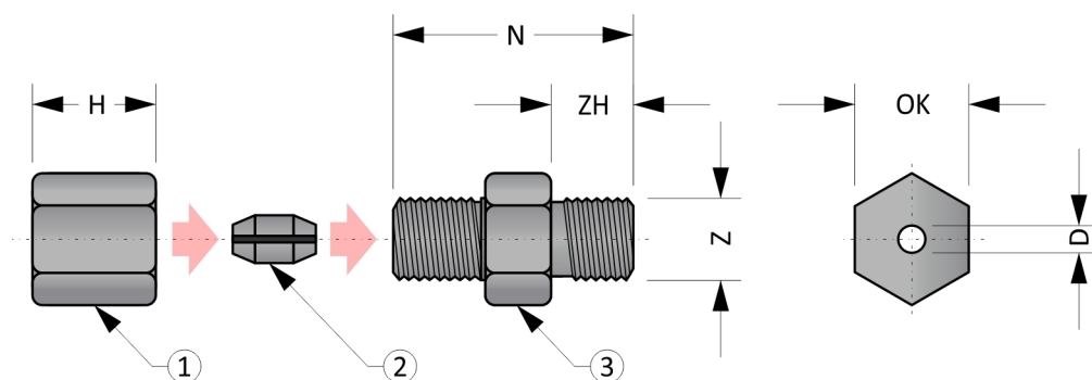
Figure PS.2: Compression fitting with C-type ferrule
