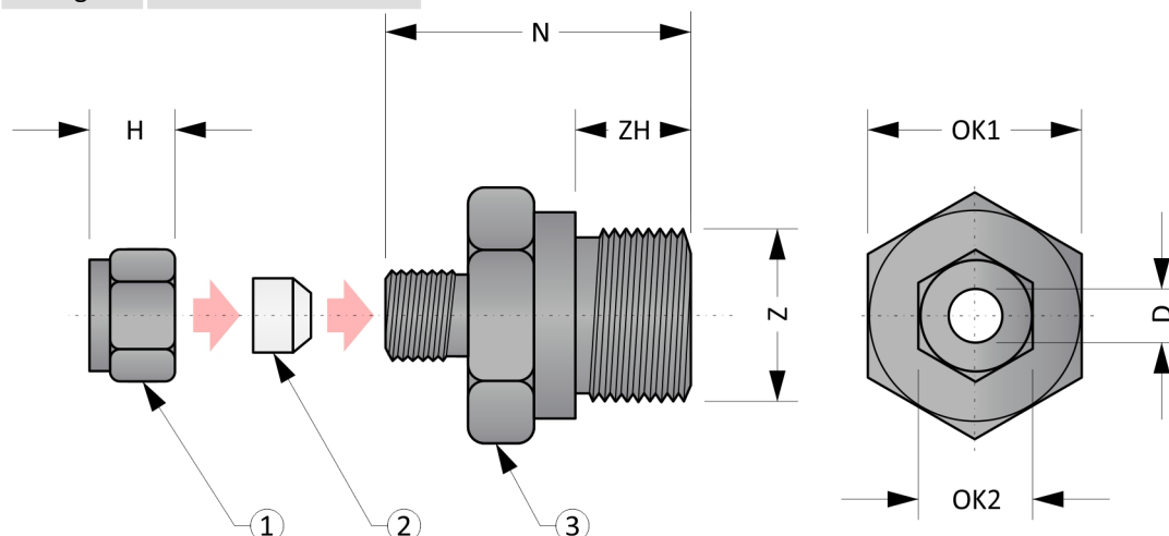
Figure PS.4: Compression fitting with Teflon ferrule
