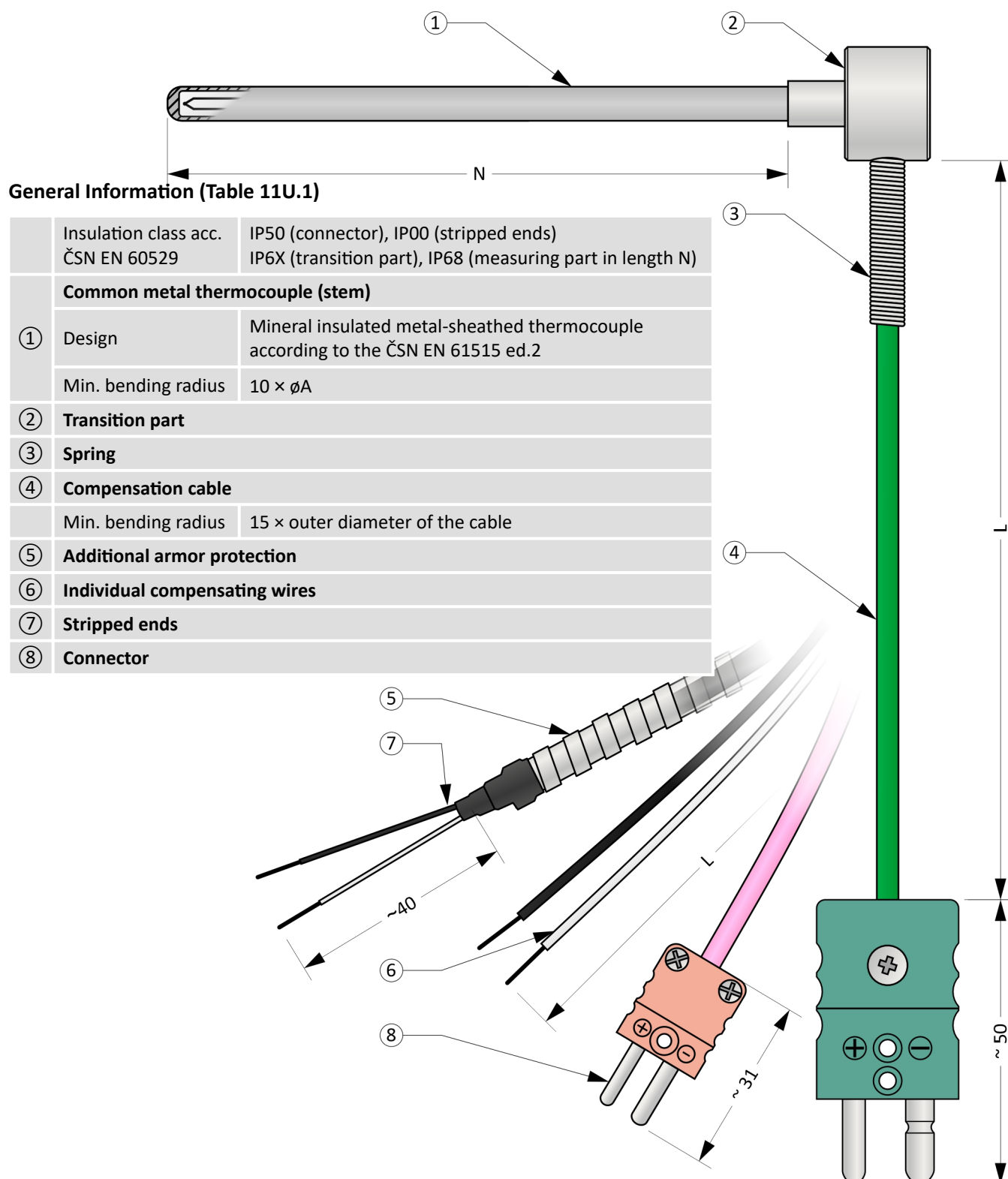
Figure 11U.1: MTC11U
