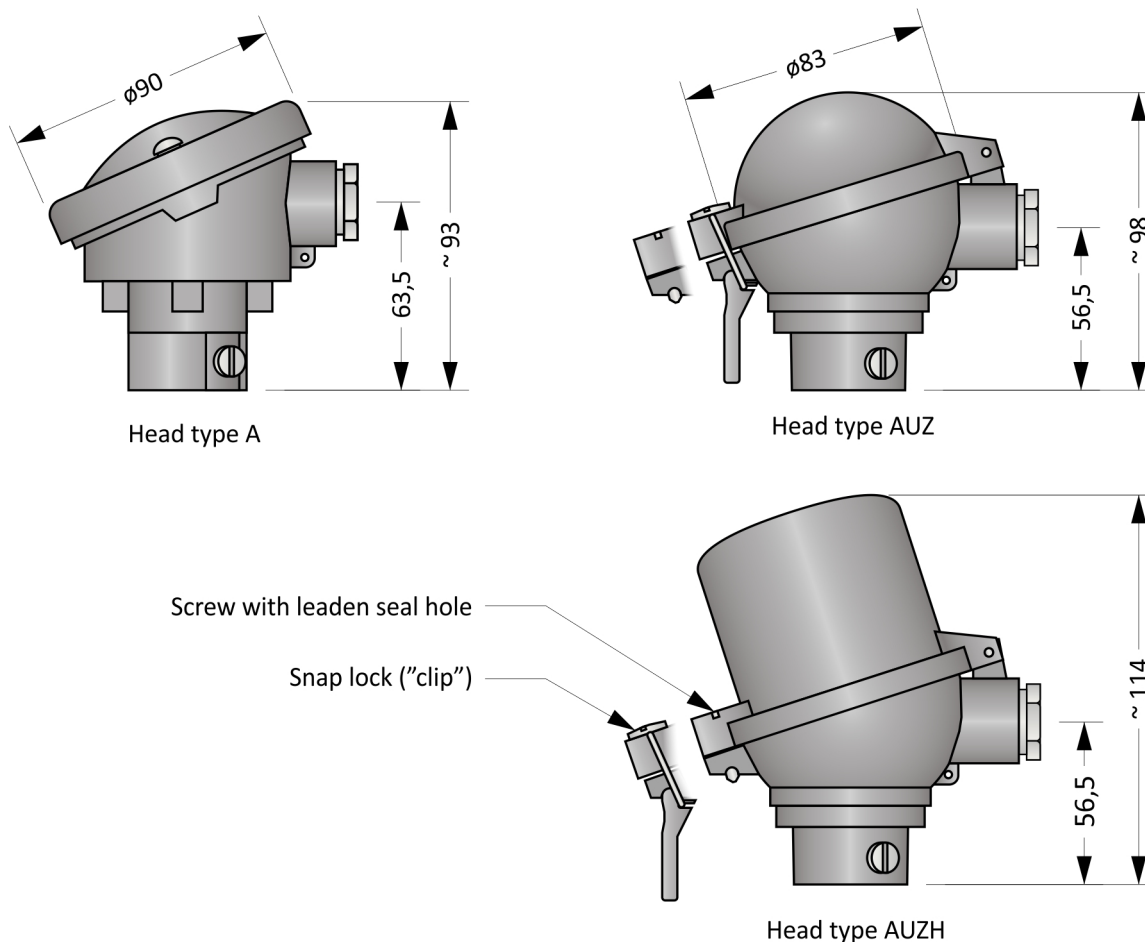
Figure 3.2: Head types
