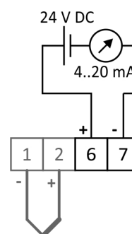
Figure 4S.4: Transmitter wiring diagram
