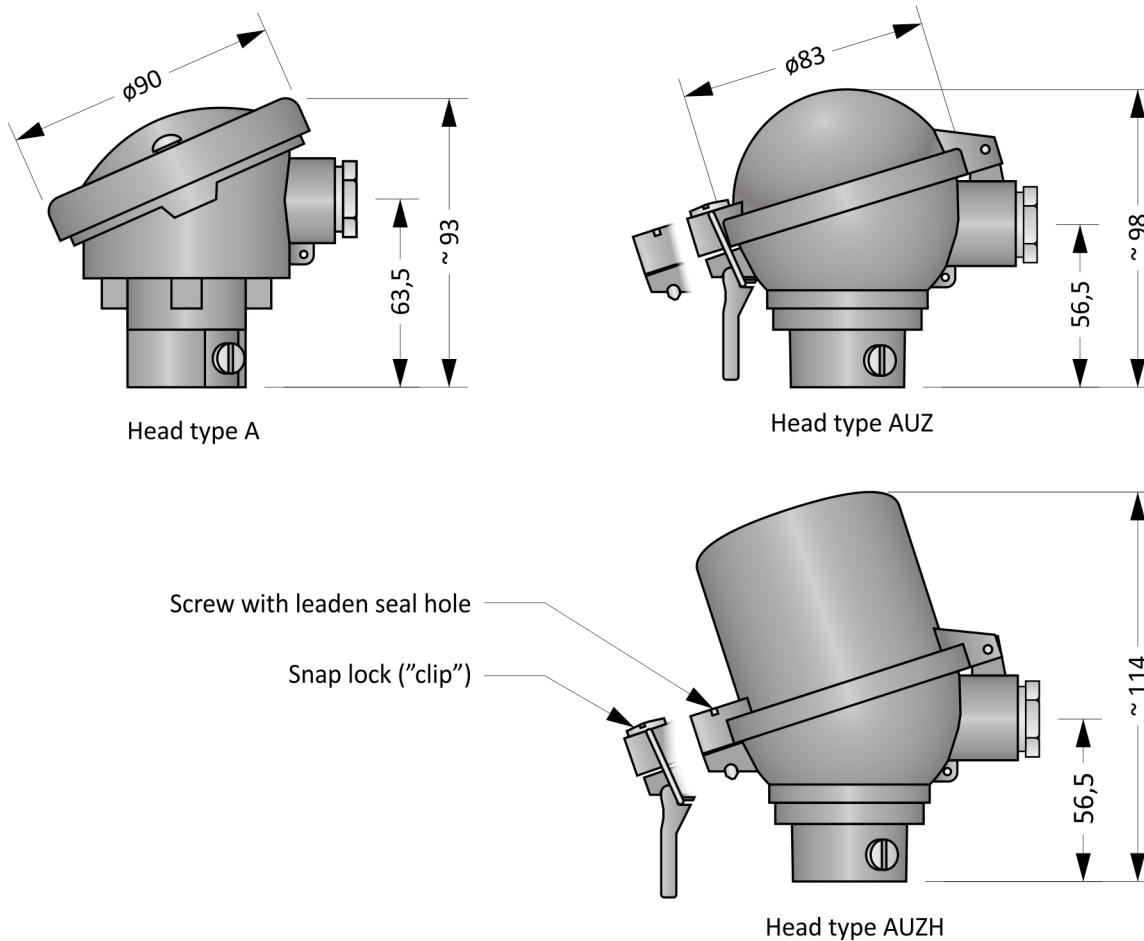
Figure 4.2: Head types
