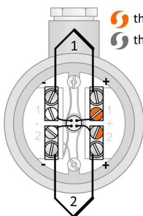
Figure 6A.3: Double thermocouple wiring diagram
